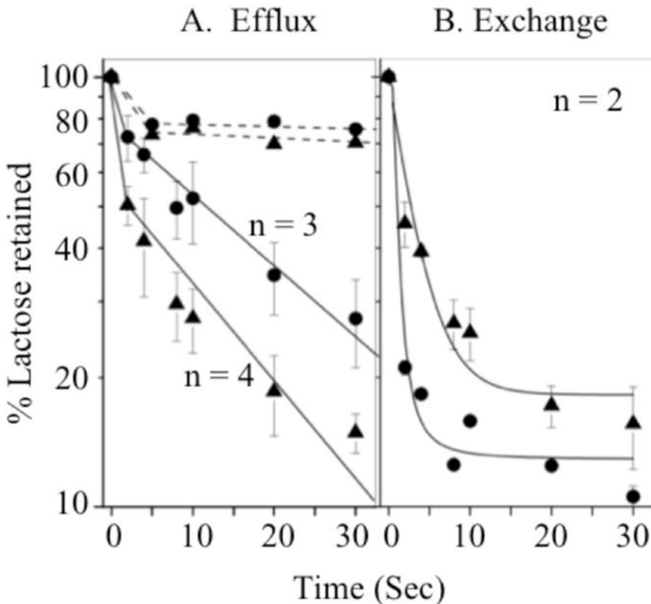
Fig. 3. Efflux and equilibrium exchange. RSO membrane vesicles containing wild type ( \lambda ) or D240E LacY ( \sigma ) in 100 mM \text{KPi} (pH 7.5) were pre-equilibrated with 10 mM [ ^{14}\text{C} ]lactose (10 mCi/mmol) in the presence of 55 \mu\text{M} valinomycin and 1 \mu\text{M} nigericin and diluted 200-fold into the same buffer in the absence (efflux) or presence (exchange) of 10 mM unlabeled lactose, and reactions were terminated by quenching and rapid filtration at given times, as described. Efflux with N -ethylmaleimide-treated RSO vesicles (10 mM, final concentration for 20 min) is indicated by broken lines. The average percentage of lactose retained is plotted as a function of time.
